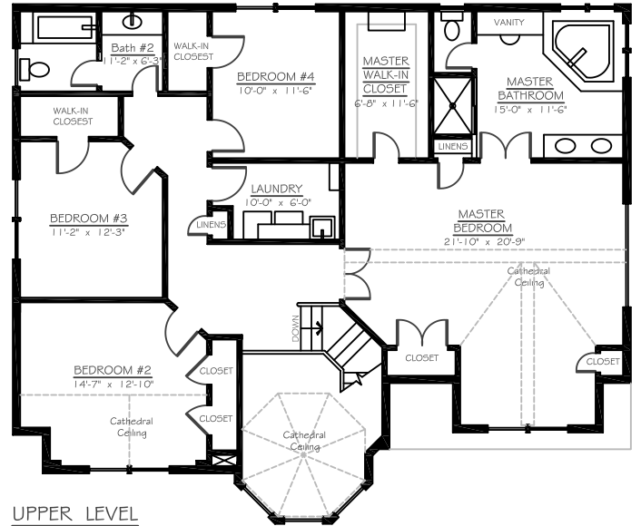
UPPER LEVEL
